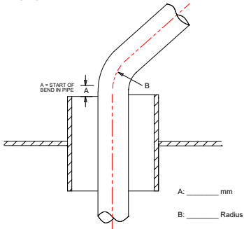
45° ELBOW - ABOVE SLEEVE
