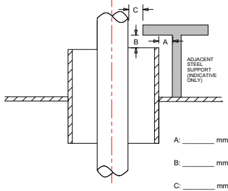
ADJACENT OBSTRUCTION
