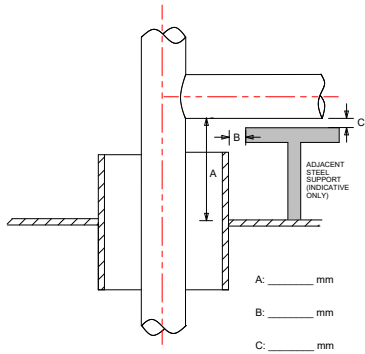
T-BRANCH HEIGHT ABOVE DECK & ADJACENT OBSTRUCTION
