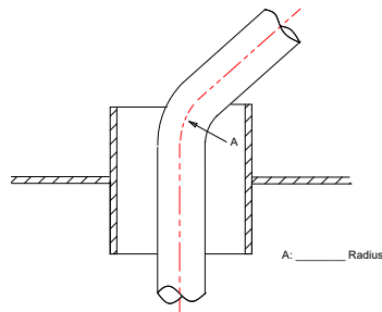
45° ELBOW - INSIDE SLEEVE
