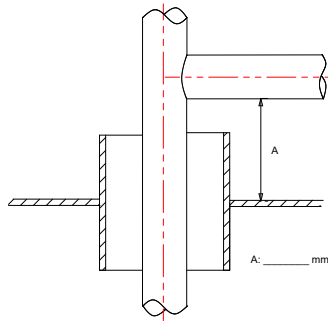
T-BRANCH HEIGHT ABOVE DECK
