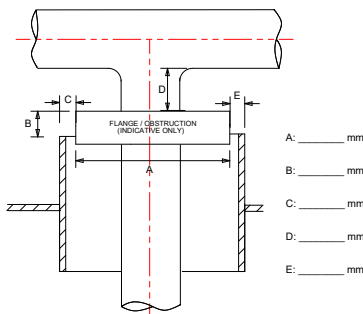
FLANGE INSIDE SLEEVE & OBSTRUCTION ABOVE
