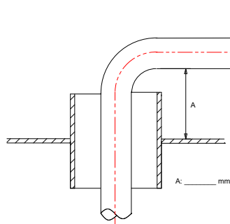
ELBOW HEIGHT ABOVE DECK
