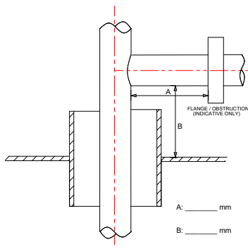
T-BRANCH HEIGHT ABOVE DECK & PIPE OBSTRUCTION
