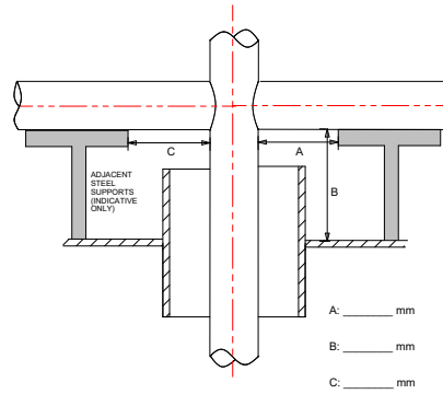
DOUBLE T-BRANCH HEIGHT ABOVE DECK & OBSTRUCTIONS
